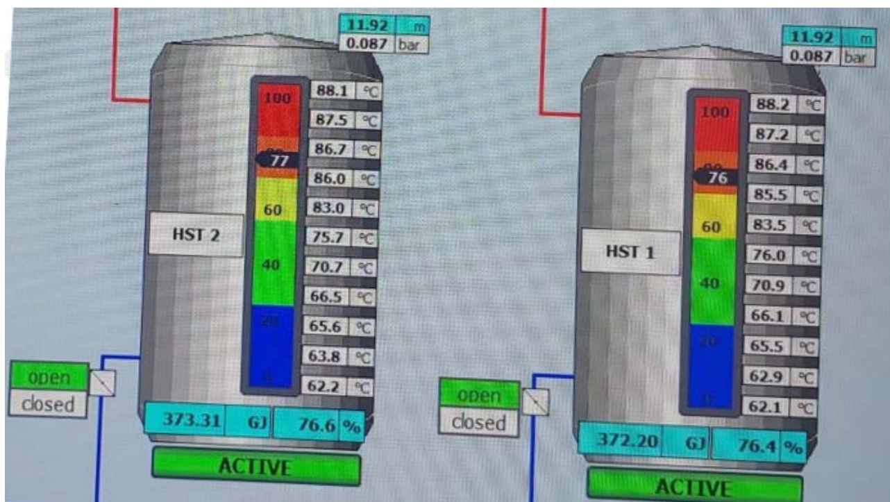
Figure 6: Human-Machine Interface (HMI) of Thermal Storage Tanks
